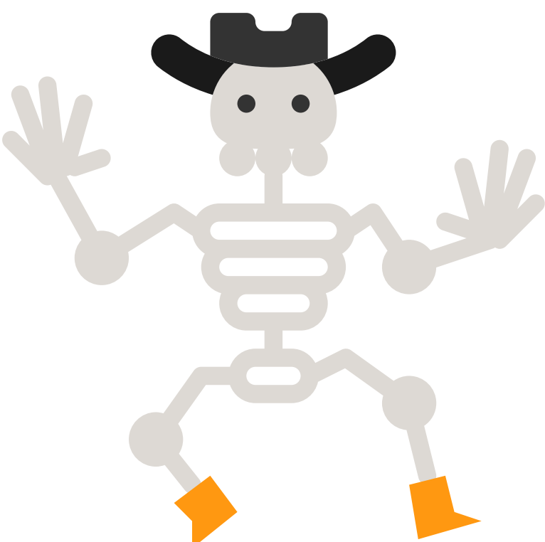
SQUELETTE
